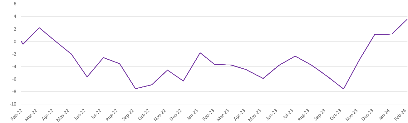
Cumulative Performance (%)*
